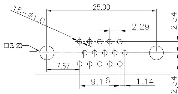
PCB Holes Diagram(Top View)
