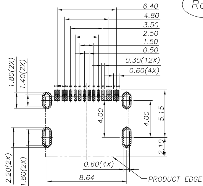
RECOMMENDED PCB LAYOUT(TOP VIEW) THICKNESS 0.60MM;DEFAULT TOLERANCE:±0.05
