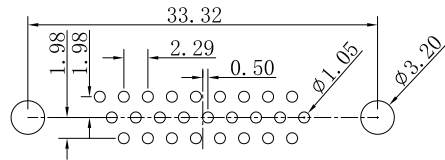
PCB layout
