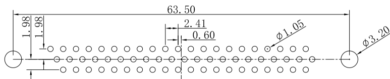
PCB layout
