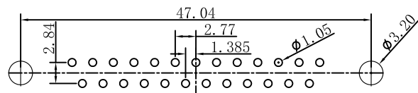
PCB layout
