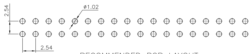
RECOMMENDED PCB LAYOUT (GENERAL TOLERANCE: ±0.05)
