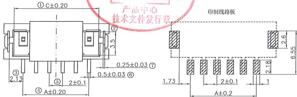
RECOMMENDED PCB Layout DEFAULT TOLERANCES:±0.05(TOP VIEW)
