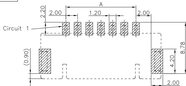
SUGGESTED PCB LAYOUT
