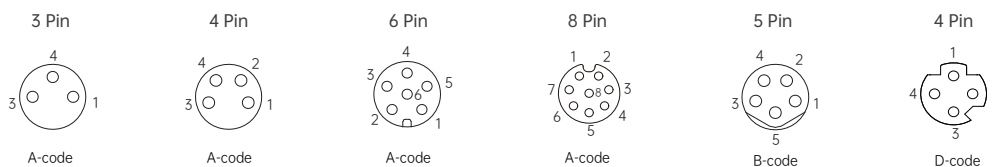
针位分布前视图 / Pin assignment front view
