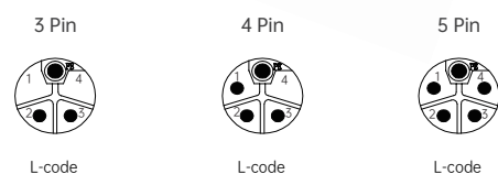
针位分布前视图 / Pin assignment front view
