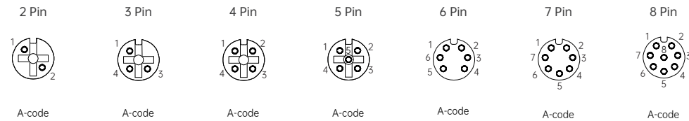
针位分布前视图 / Pin assignment front view
