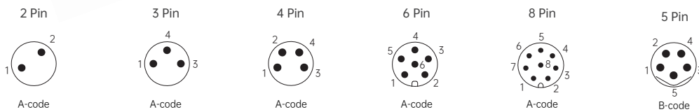
针位分布前视图 / Pin assignment front view
