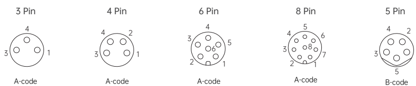
针位分布前视图 / Pin assignment front view
