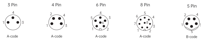
针位分布前视图 / Pin assignment front view
