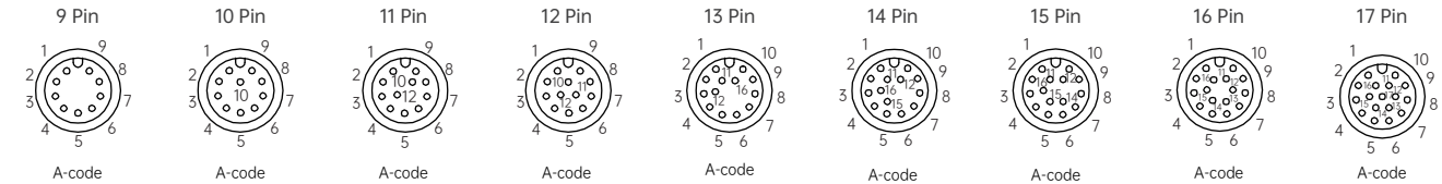
针位分布前视图 / Pin assignment front view
