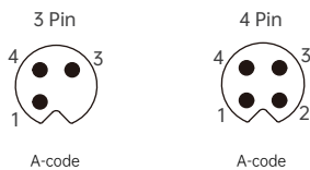
针位分布前视图 / Pin assignment front view
