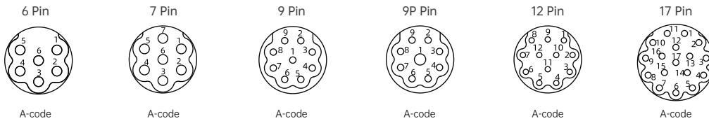
针位分布前视图 / Pin assignment front view
