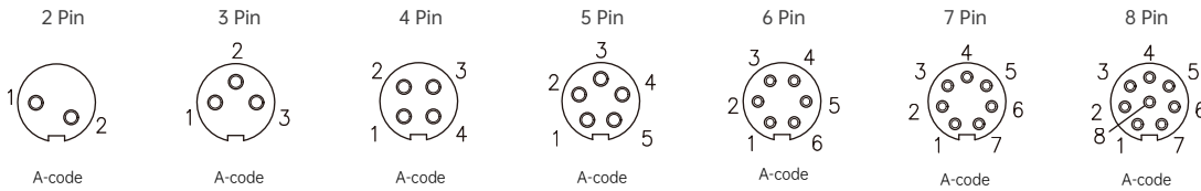
针位分布前视图 / Pin assignment front view
