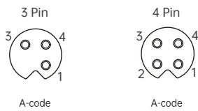
针位分布前视图 / Pin assignment front view
