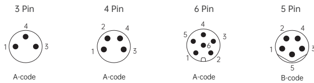
针位分布前视图 / Pin assignment front view
