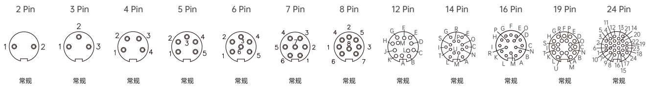
针位分布前视图 / Pin assignment front view
