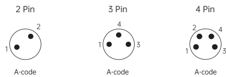
针位分布前视图 / Pin assignment front view
