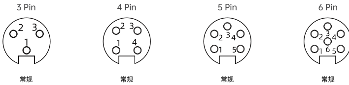
针位分布前视图 / Pin assignment front view
