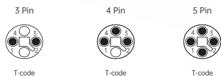
针位分布前视图 / Pin assignment front view
