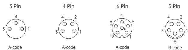
针位分布前视图 / Pin assignment front view
