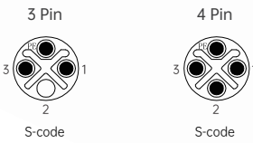
针位分布前视图 / Pin assignment front view
